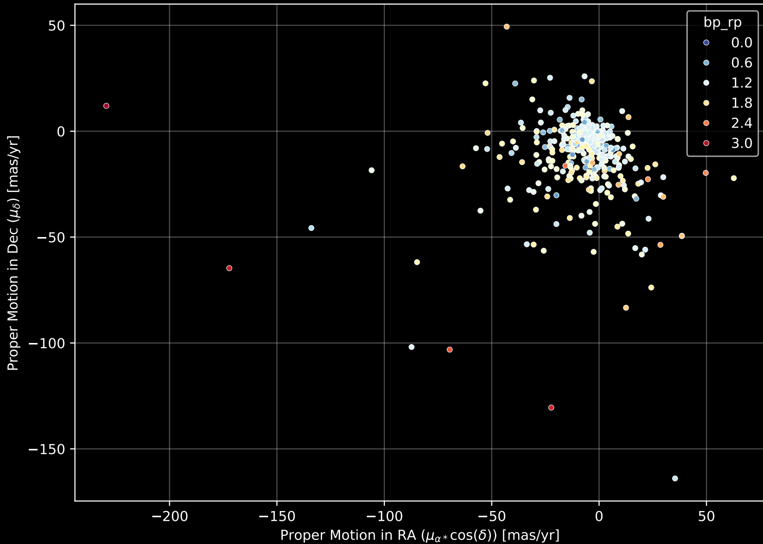
APOGEE DR17 Field: [M67] Proper Motion Diagram (n= 588)
