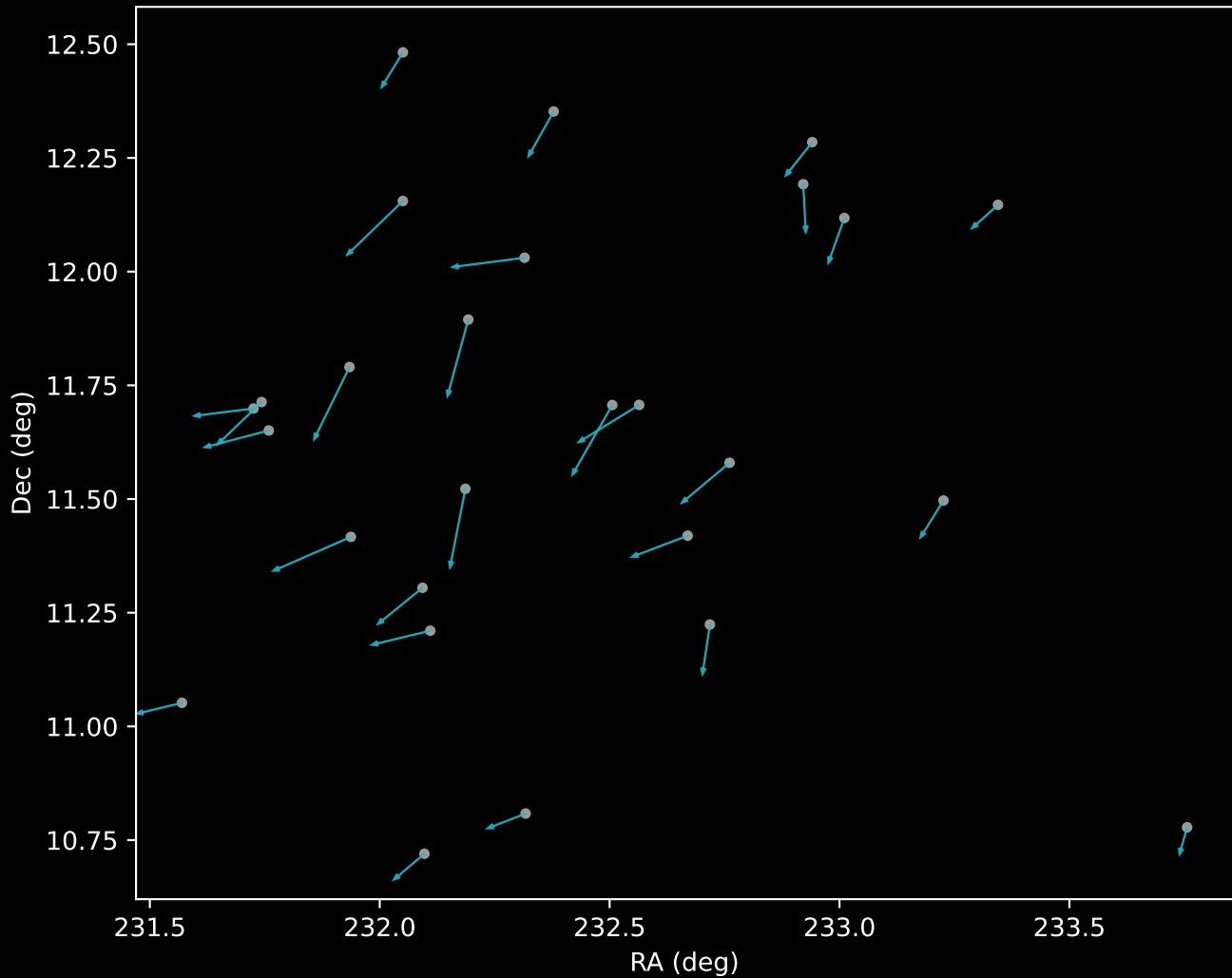
APOGEE DR17 Cluster 18 Proper Motion Vectors (n=27)
