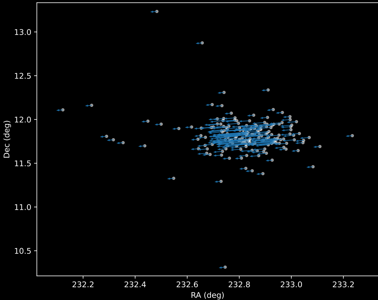
APOGEE DR17 Cluster 20 Proper Motion Vectors (n=176)
