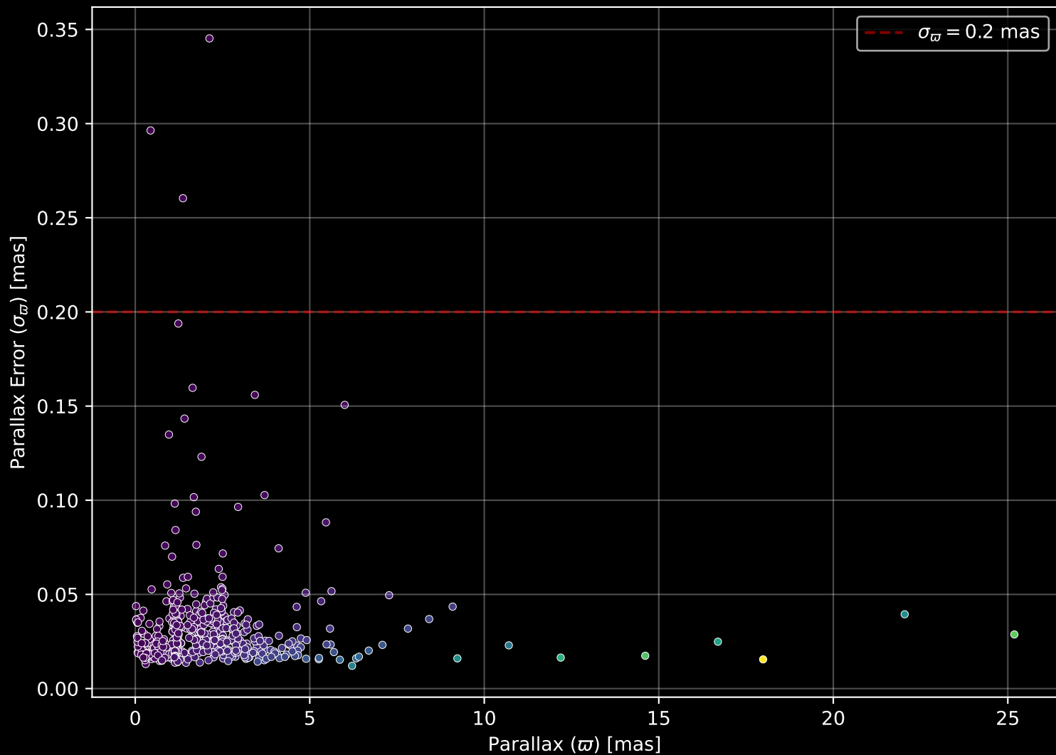
APOGEE DR17 Field: [M67] Parallax Quality (n= 588)
