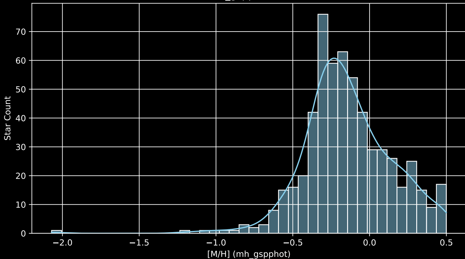
APOGEE DR17 Field: [M67 [M/H] (mh_gspphot) (n= 575)
