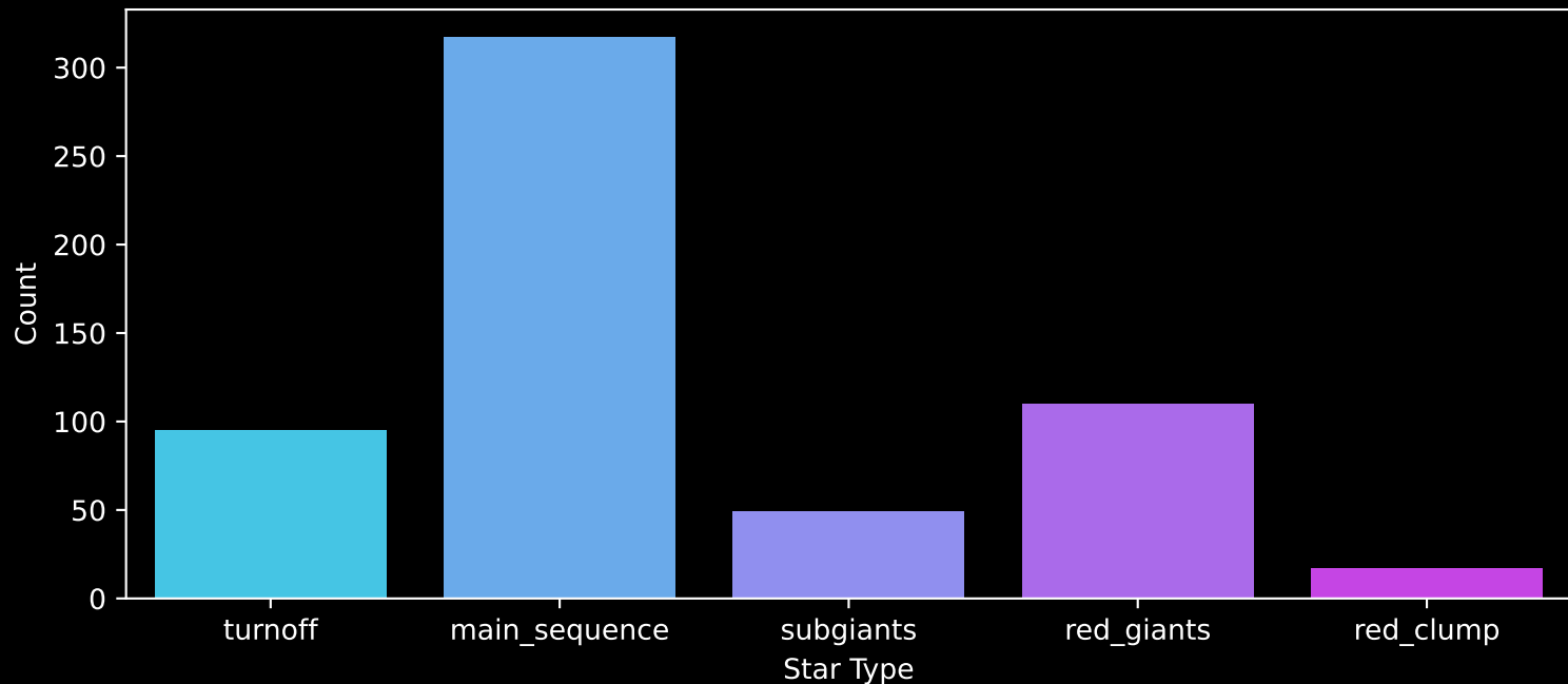
APOGEE DR17 Field: [M67] Count plot of Star Type
