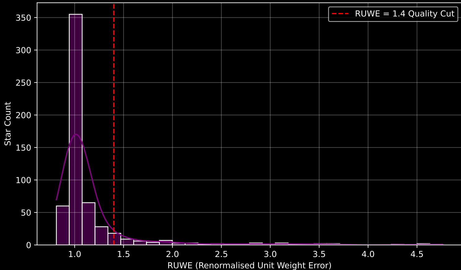
GAPOGEE DR17 Field [M67] RUWE Distribution (n= 579)
